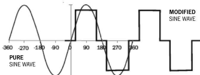
Figure 1: Modified Sine Wave and Pure Sine Wave Comparison
